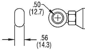
CLEVIS EYEBOLT
